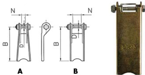
SPRING SAFETY LATCH FOR HOOKS
